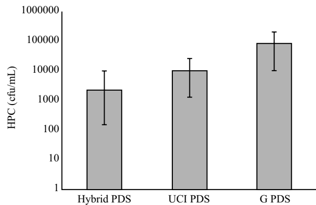
Figure 8 | Effluent HPC concentrations for hybrid, unlined cast iron, and galvanized steel pilot distribution systems (RZA method, 9/09/02–12/20/02, observations = 8).
