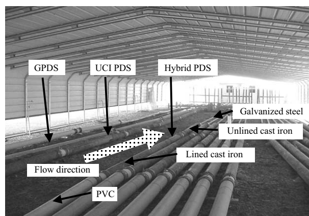
Figure 1 | Polyvinyl chloride (PVC), lined cast iron (LCI), unlined cast iron (LCI) and galvanized steel (G) pilot distribution systems.
