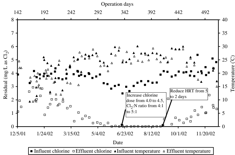
Figure 5 | Hybrid pilot distribution system total residual and temperature during operation.
