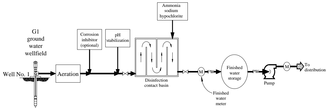
Figure 2 | The conceptual schematic design of groundwater treatment process.
