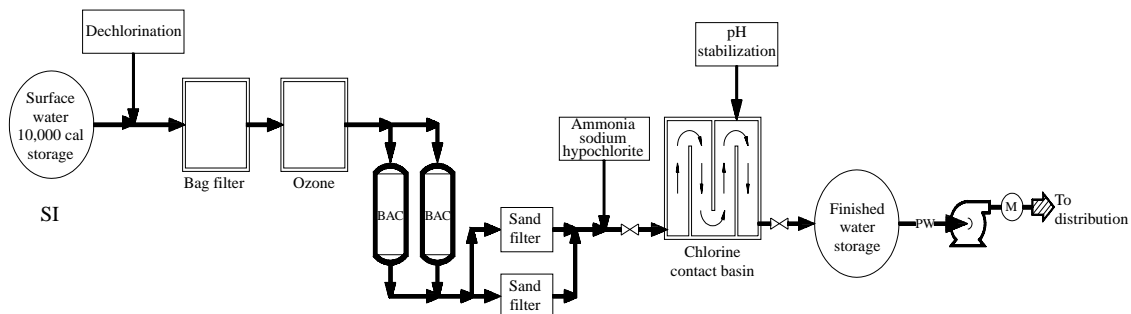
Figure 3 | The conceptual schematic design of surface water treatment process.
