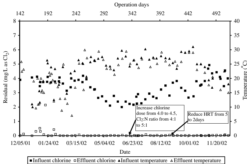
Figure 7 | Galvanized steel pilot distribution system total residual and temperature during operation.
