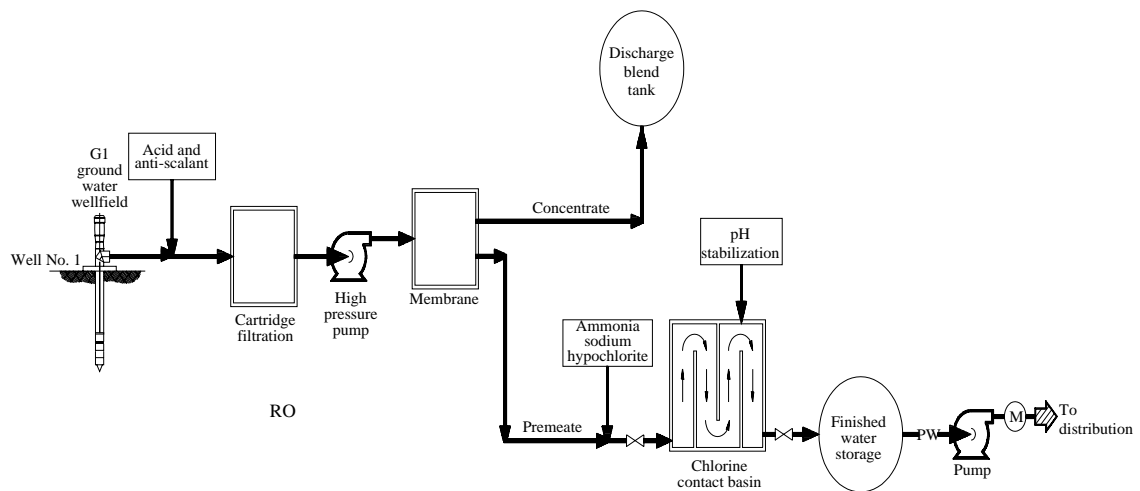
Figure 4 | The conceptual schematic design of desalination treatment process.
