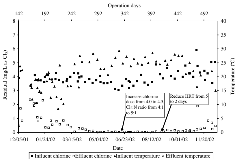
Figure 6 | Unlined cast iron pilot distribution system total residual and temperature during operation.
